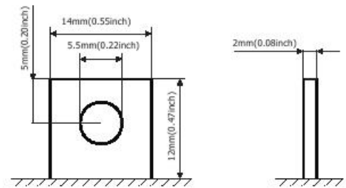
Terminal Dimensions
