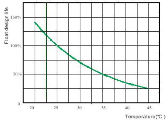
Temperature vs design life curve
