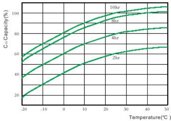
Temperature vs capacity curve
