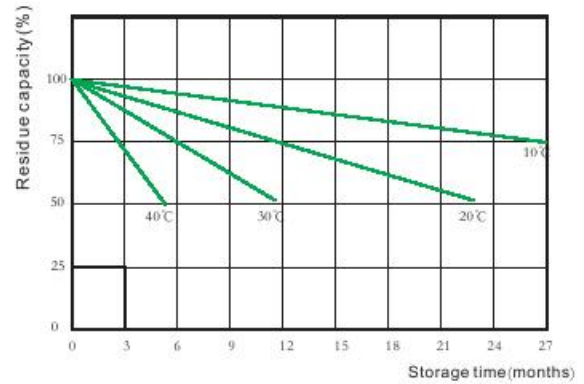
Residue capacity vs. storage time
