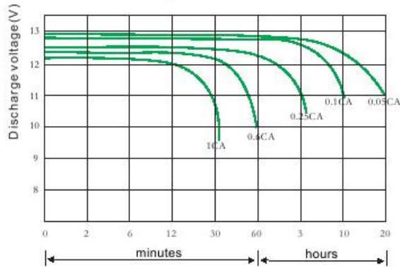
Discharge curve ( 25°C )
