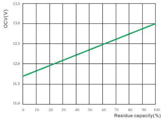
OCV vs state of charge
